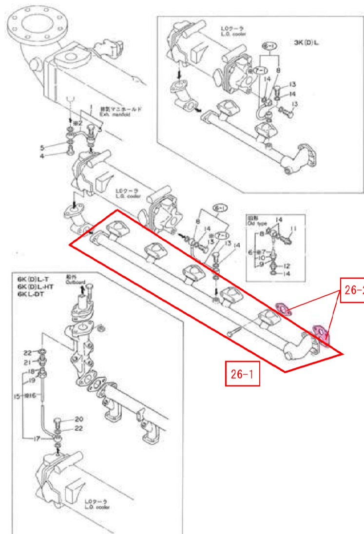
CW管 (LOクーラ〜排気マニホールド・CW分配管・出口連絡管) COOLING WATER PIPE (L.O. COOLER-EXH. MANIFOLD・C.W. DISTRIBUTING PIPE-OUTLET CONNECTING PIPE)
